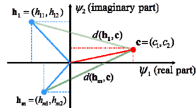
Fig. 4. The example of Euclidean distance.
