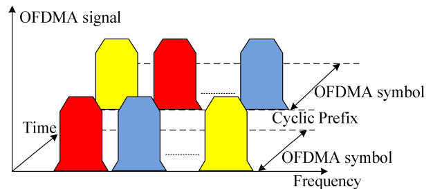
Fig. 1. OFDMA signal in frequency and time domain.
