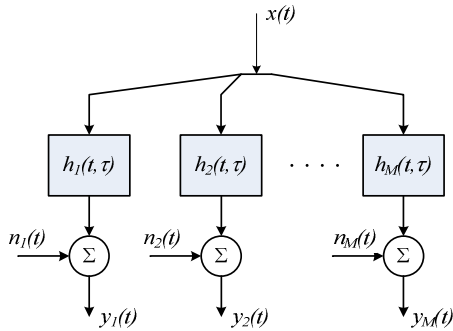
Fig. 5. Channel model.
